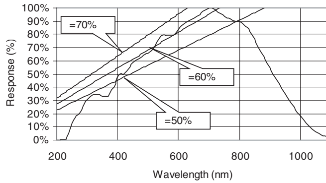
Figure 1-1. Spectral Response
