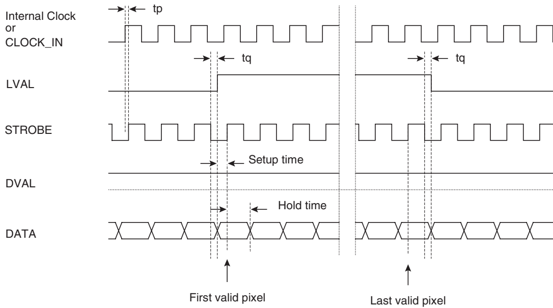
Figure 6-6. Timing Diagram at Camera Link Device Input
