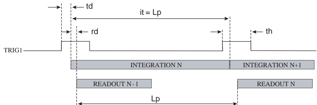
Figure 6-5. Triggered Readout Mode Timing Diagram
