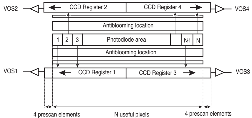
Figure 2-1. CCD Architecture
