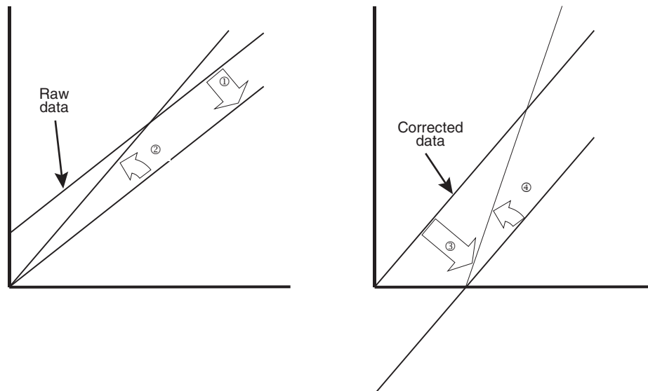
Figure 2-5. FCC and Contrast Expansion
