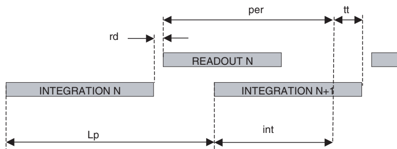
Figure 6-1. Free-run Mode Timing Diagram
