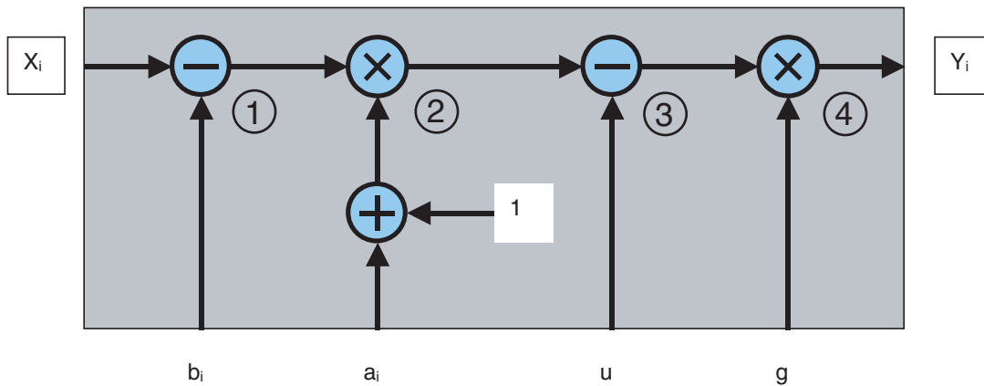
Figure 2-4. Digital Signal Processing
