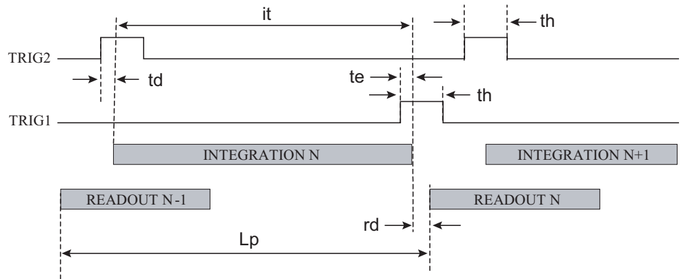
Figure 6-4. ITC Mode with Two Signals Timing Diagram
