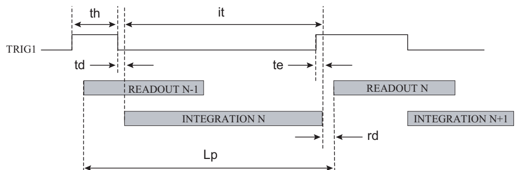
Figure 6-3. ITC Mode with One Signal Timing Diagram
