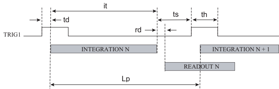
Figure 6-2. Triggered Mode Timing Diagram
